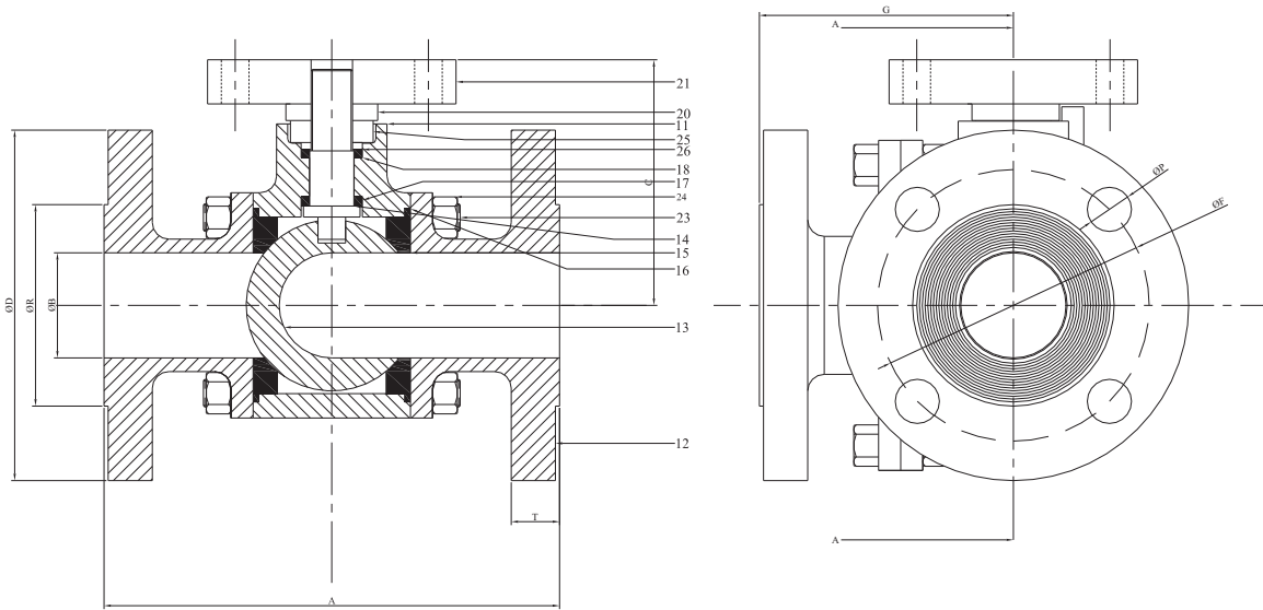
SECTIONAL VIEW A-A
