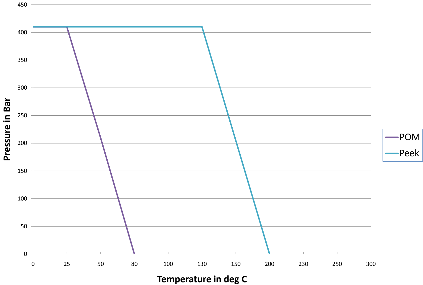
Temperature v/s Pressure Chart for POM and Peek seat Materials
