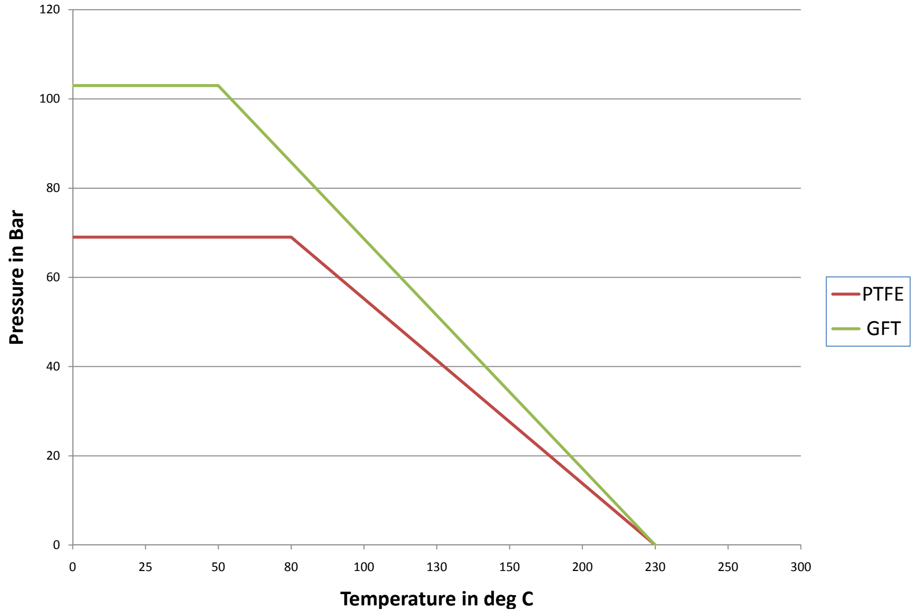
Temperature v/s Pressure Chart for PTFE and GFT seat Materials
